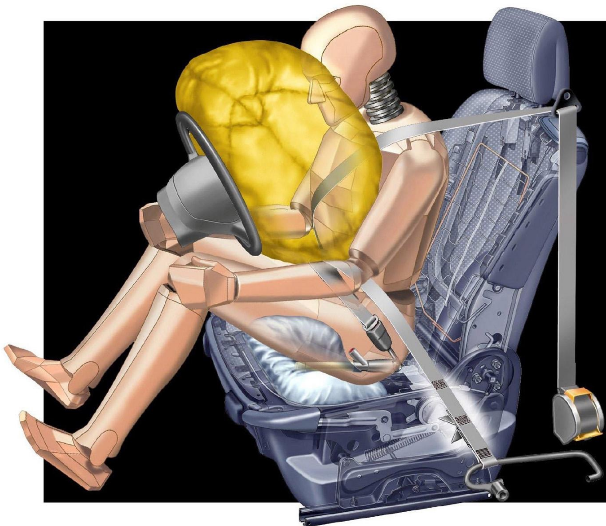
ANTI-DIVE AIRBAG
